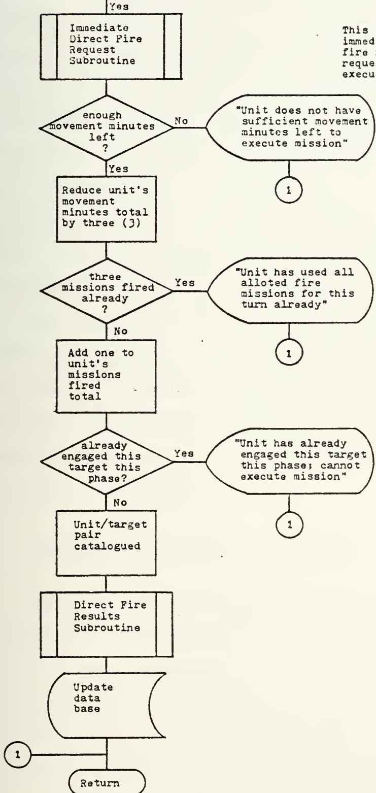
FIGURE VI.1 FLOWCHART OF IMMEDIATE DIRECT FIRE REQUEST SUBROUTINE
